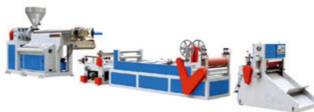
☑ SX3-D-PP, PS SHEET EXTRUDER UNIT MOULD 1500
