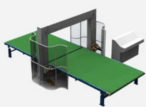
CNC Oscillating Blade Contour Cutter
