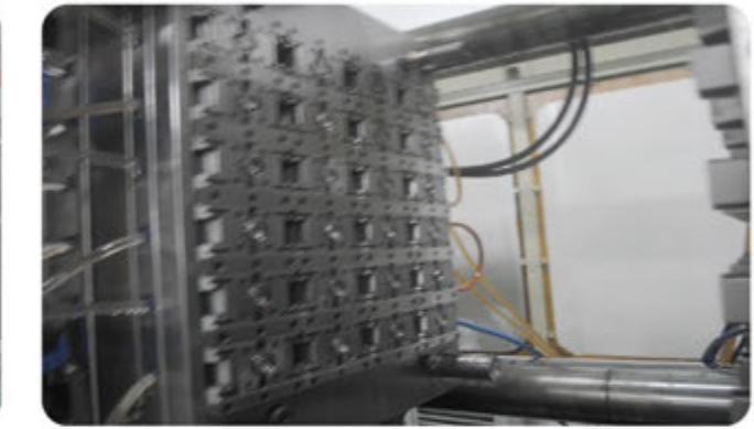
24-cavity injection cap mold
