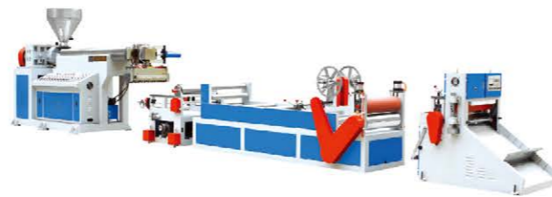
☑ SX3-D-PP, PS SHEET EXTRUDER UNIT MODEL 1500
