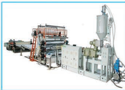
PE防水片材（土工膜）挤出生产线 PE Water Proof Sheet (Geomembrane) Extrusion Line
