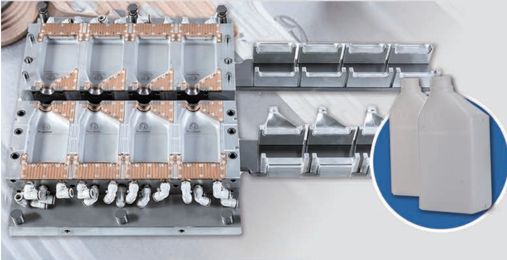
Jerrycan Blow Mould
