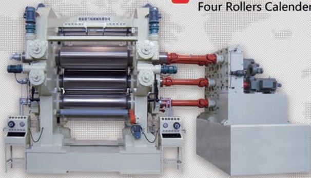
压延机 Four Rollers Calendar
