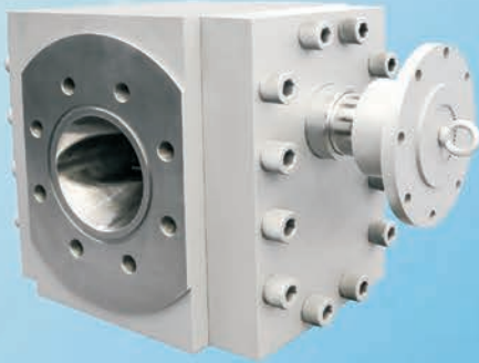
Melt Pump
