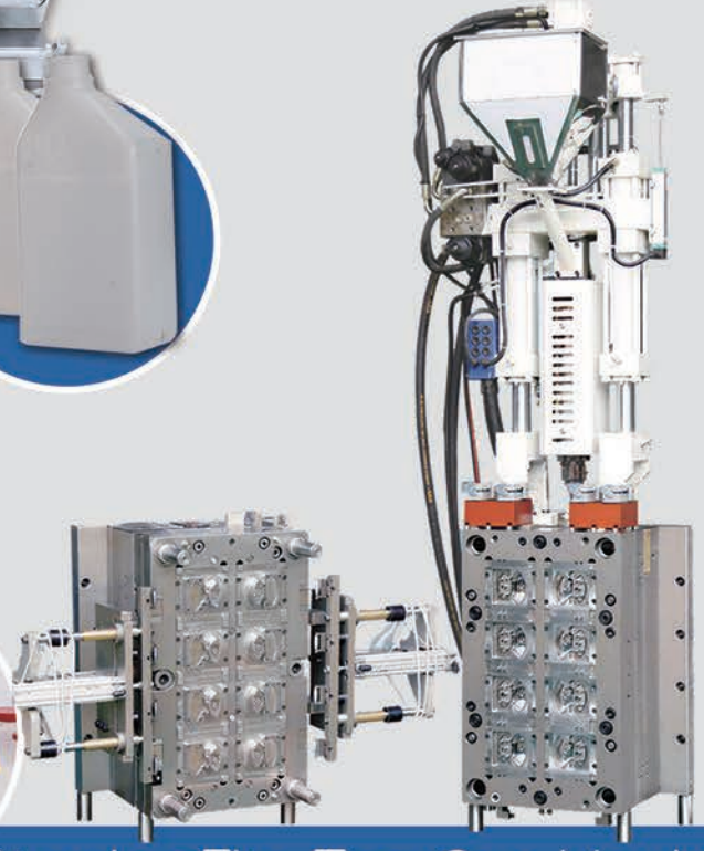
Bi-color Flip-Top Cap Mould
