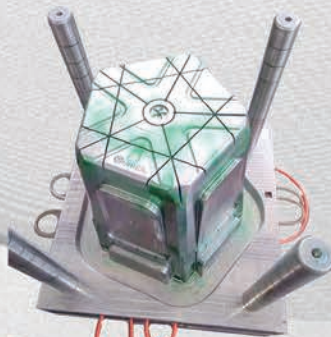
▲ Stool Mould
