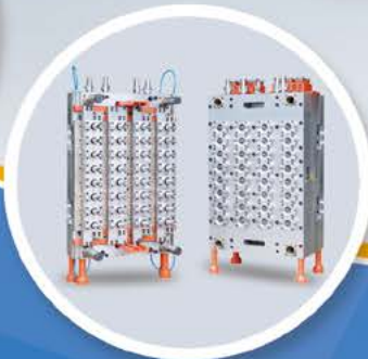
32 CAVITY HOT RUNNER PET OIL PREFORM MOULD
